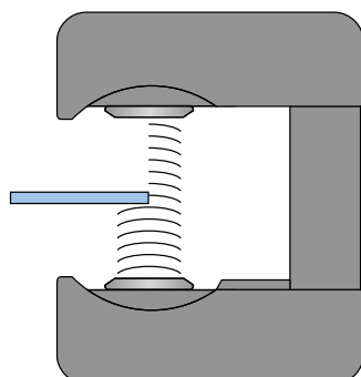
Principle of operation FX 42
