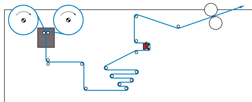
ELGUIDER DRS07 on packaging machine
