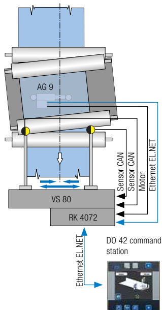
Web guiding system with sensor positioning and command station
