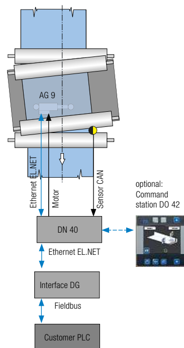
Web guiding system with interface module
