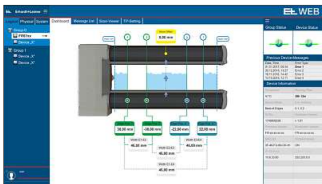
Parameter view, wide band sensor
