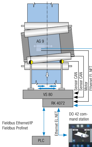
Web guiding system with sensor positioning and standard interface
