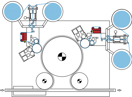
ELGUIDER DRB14 on labeling machine
