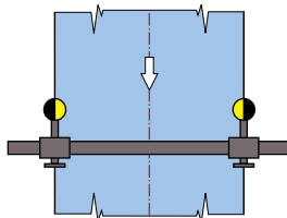
Guiding by the ideal web center line/machine center line
