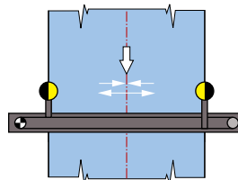
Guiding by the ideal web center line/machine center line with symmetric sensor positioning (hybrid control)
