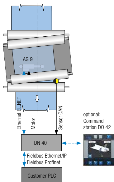
Web guiding system with standard interface Ethernet/IP/Profinet
