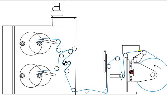
ELWINDER WSB90 on slitter rewinder
