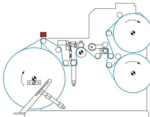
ELWINDER WSB91 on slitter rewinder
