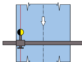
Guiding by a printed line or existing contrasts
