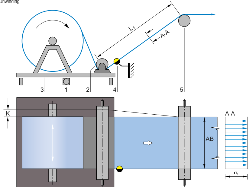
Unwinding
