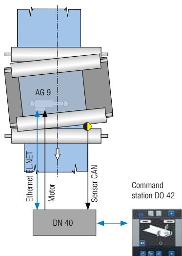
Web guiding system with command station
