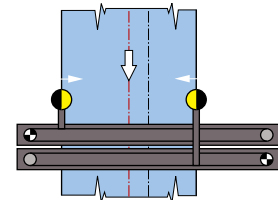
Guiding by the web center which does not correspond to the machine center with motorized sensor positioning for both sides (automatic edge search)
