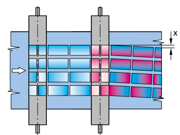
Printed image travel
