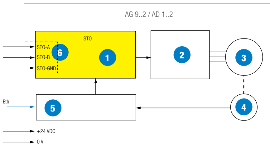
Simplified block diagram of the BLDC drive: 1 Impulse block / 2 Power stage / 3 Motor / 4 Multitrans encoder / 5 Drive control / 6 Galvanic isolation
