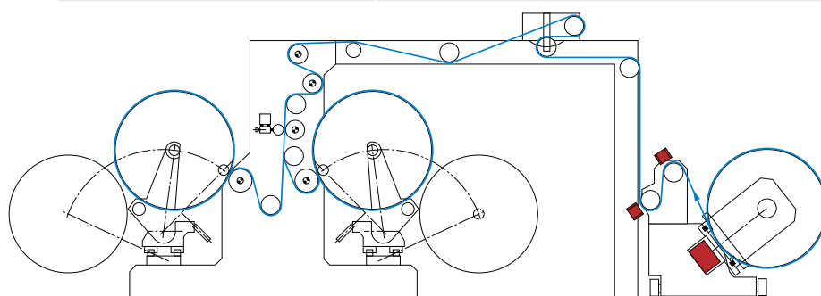
ELWINDER WSB96 on slitter rewinder
