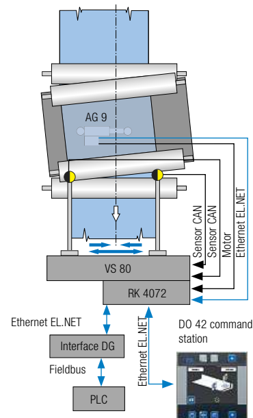
Web guiding system with sensor positioning and interface module
